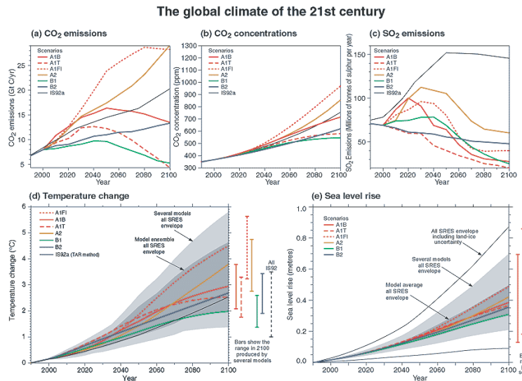
Future climate depends on natural changes and human activities.
