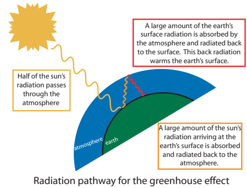
Radiation pathway for the greenhouse effect
