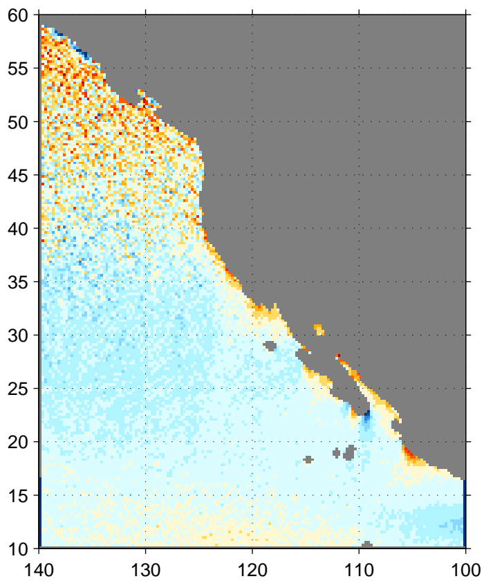
Climatological DJF pseudostress curl ( \text{m/s}^2 \cdot 1.0\text{e}6 ) (QuikScat)
