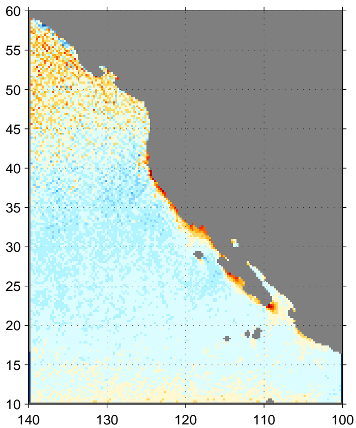
Climatological SON pseudostress curl ( \text{m/s}^2 \cdot 1.0\text{e}6 ) (QuikScat)
