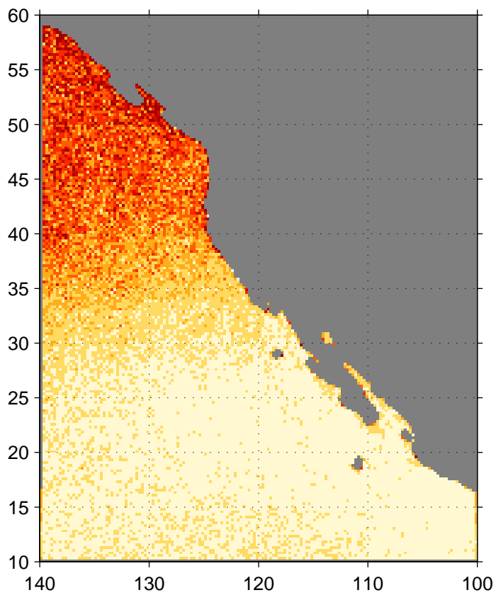
Standard deviation of DJF-mean pseudostress curl ( \text{m/s}^2 \cdot 1.0\text{e}6 ) (QuikScat)
