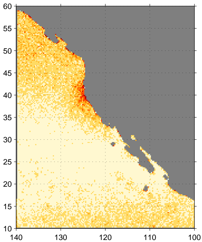
Standard deviation of JJA-mean pseudostress curl ( \text{m/s}^2 \cdot 1.0\text{e}6 ) (QuikScat)
