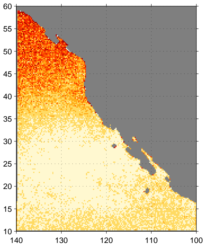
Standard deviation of MAM-mean pseudostress curl ( \text{m/s}^2 \cdot 1.0\text{e}6 ) (QuikScat)
