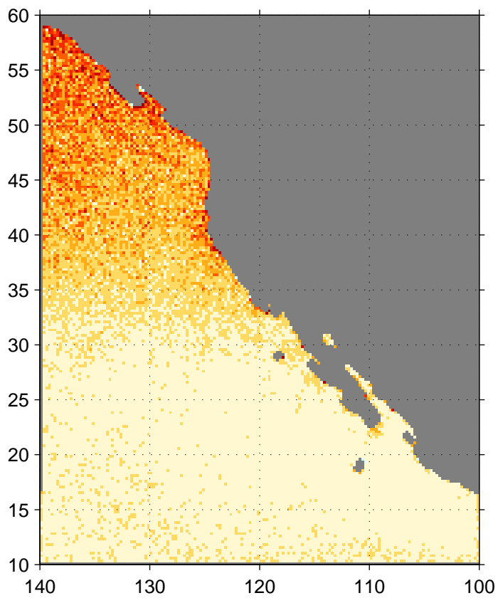
Standard deviation of SON-mean pseudostress curl ( \text{m/s}^2 \cdot 1.0\text{e}6 ) (QuikScat)
