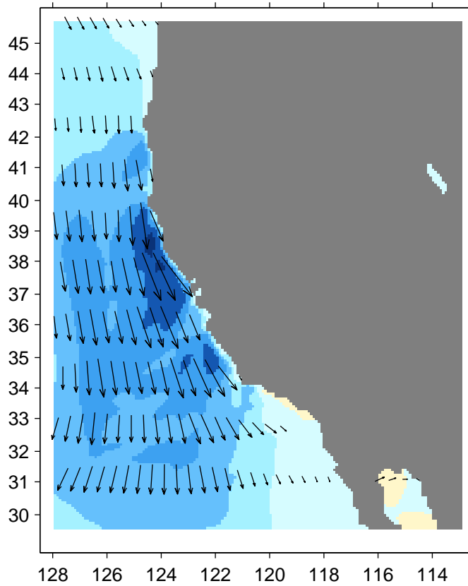
CaRD10, version 1 mid-August 2000 (hour 5427) vector pseudostress and meridional pseudostress (shaded, m 2 /s 2 )
